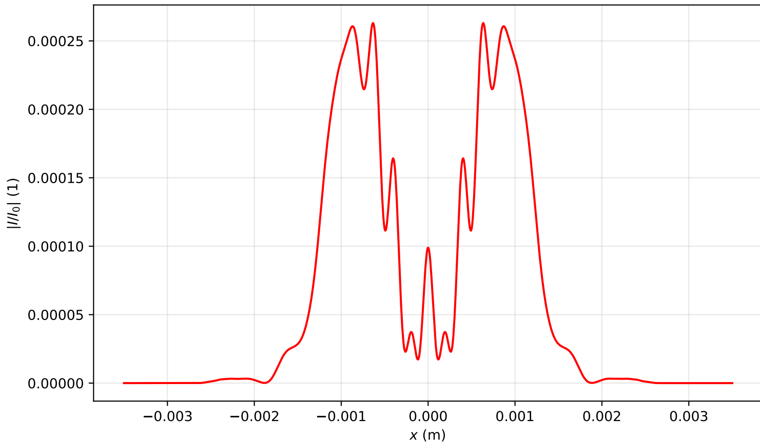
Intensity profile I(x, y = 0, z = 1.035)/I_0 , P_{in}=9.0P_{cr} , artificial time
